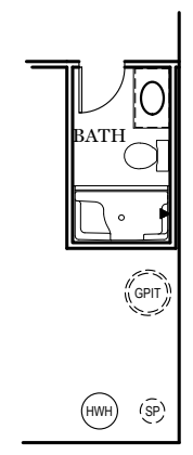
OPTIONAL FINISHED BATHROOM (+ 52 SF)
