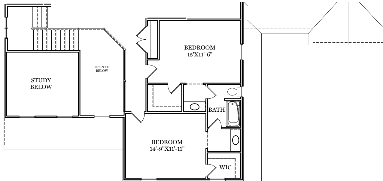
HOMESTEAD FLOOR PLAN
